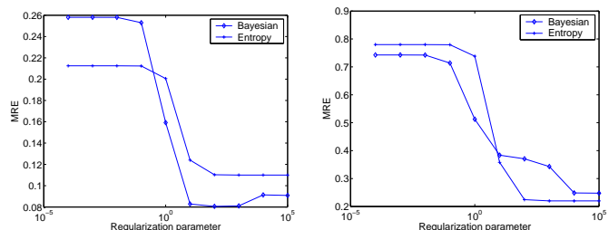
Figure 13: Mean relative error (MRE) as a function of the regularization parameter for the European network (left) and the American network (right).
